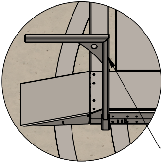
DETAIL D SCALE 1 : 28
