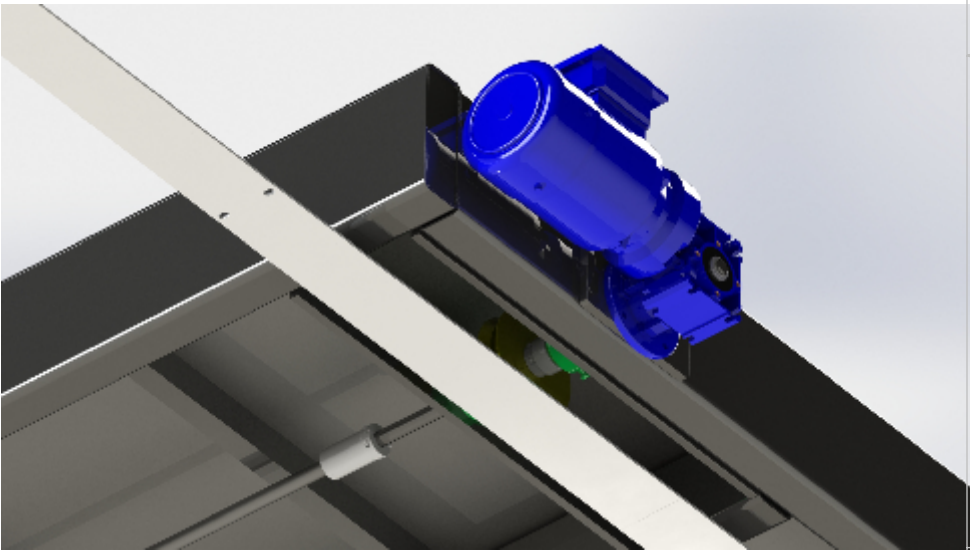
BOTTOM MOTOR/DRIVE SHAFT VIEW
