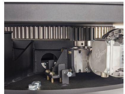
QUALITY SLEWING DRIVE AND PINION GEAR
