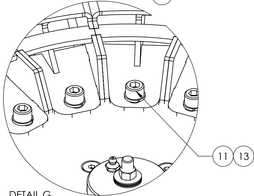
DETAIL G SCALE 1 : 2
