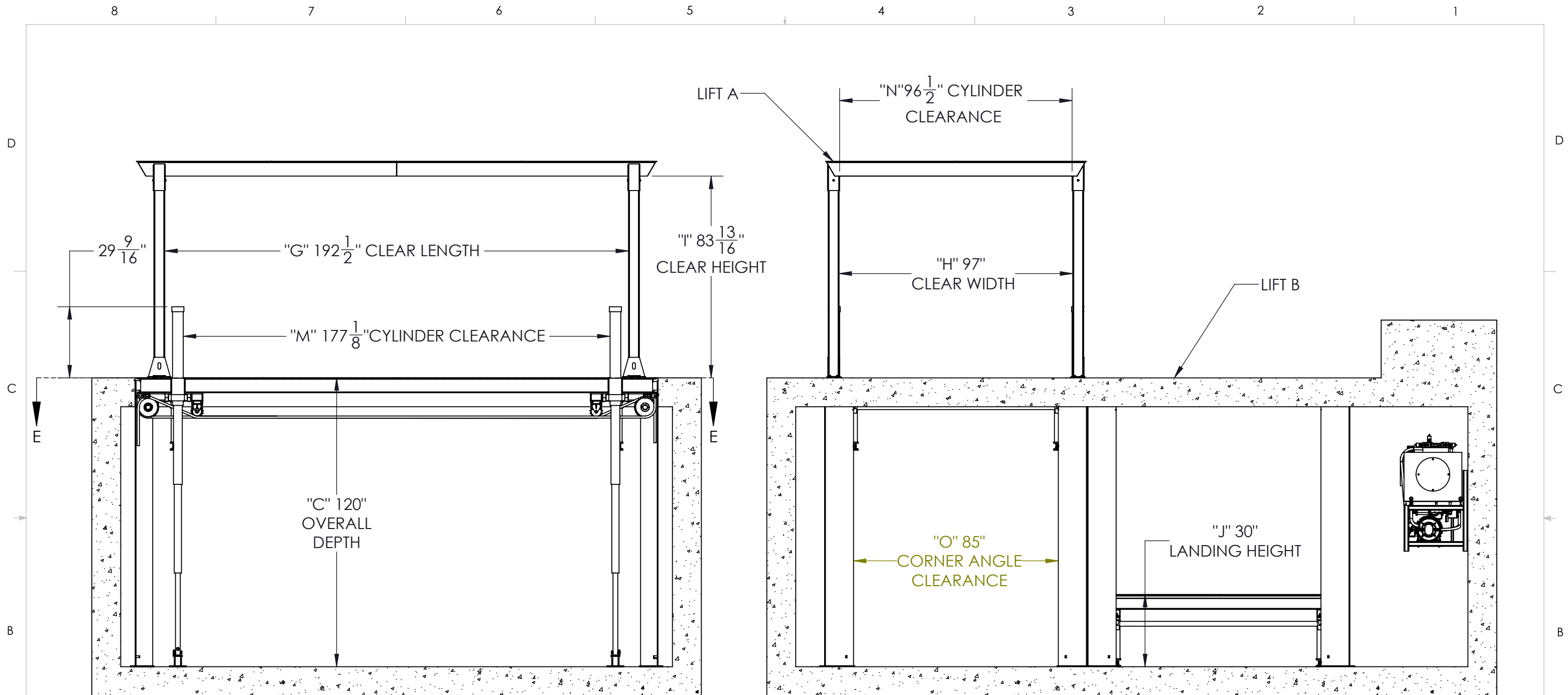
ELEVATION VIEW LIFT A RAISED POSITION (LIFT B NOT SHOWN FOR CLARITY)
