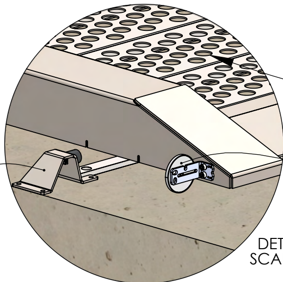
DETAIL M SCALE 1 : 4
