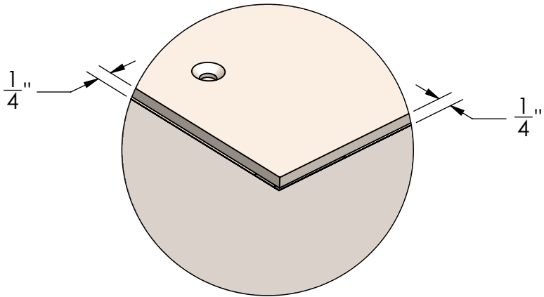
DETAIL D MOTOR COVER GAP SCALE 1 : 2
