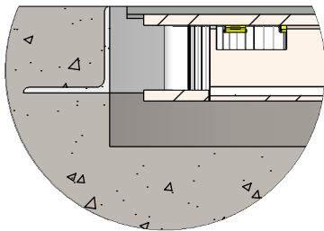
DETAIL H SCALE 1 : 4
